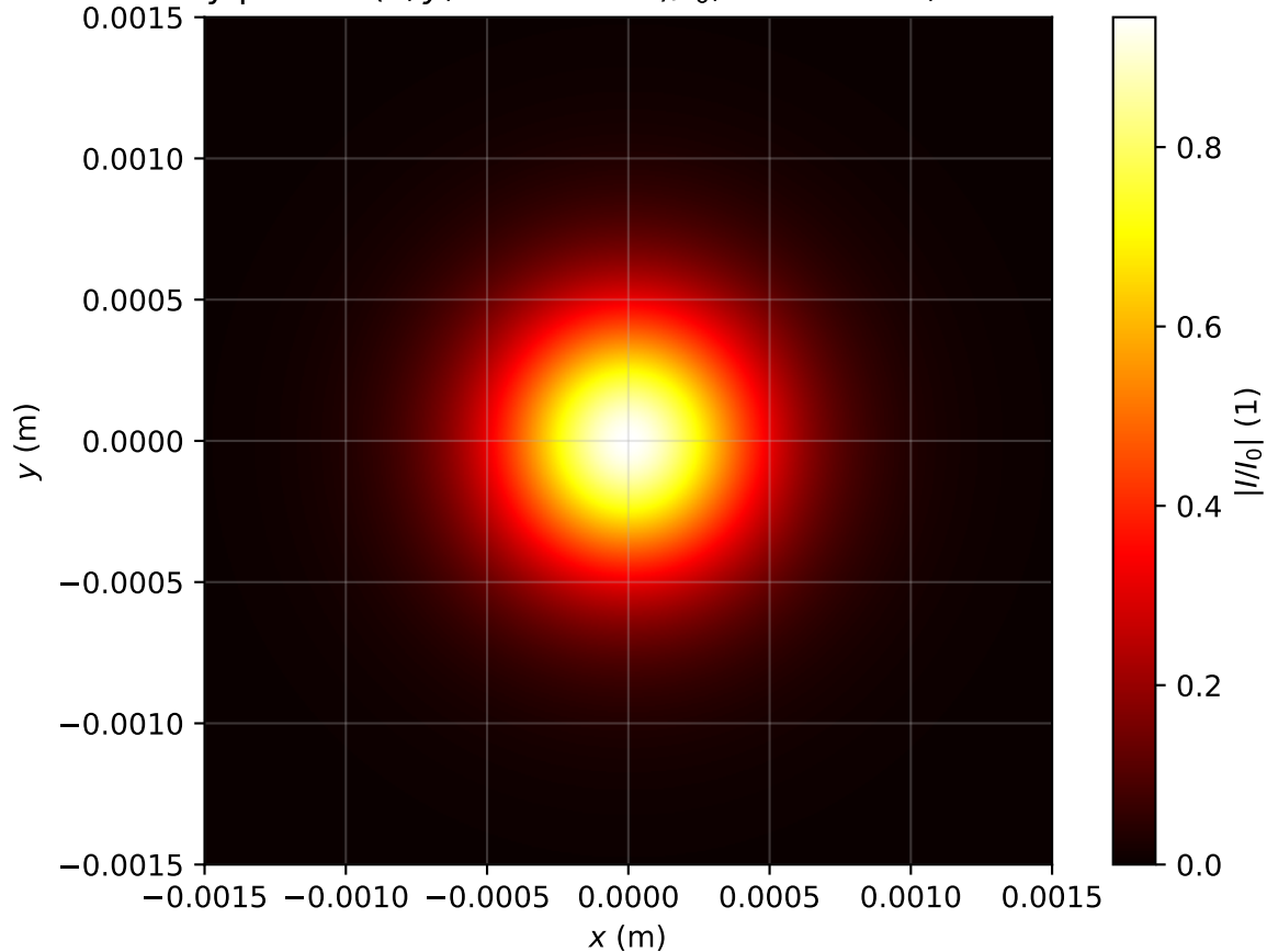
Intensity profile I(x, y, z = 1.990m)/I_0 , P_{in}=0.6P_{cr} , artificial time
